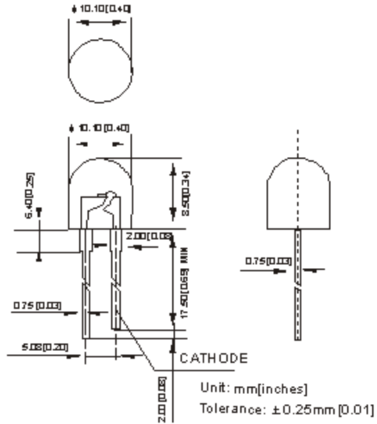
Package Dimensions
